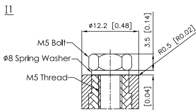
Detail A Drawing(4:1)
